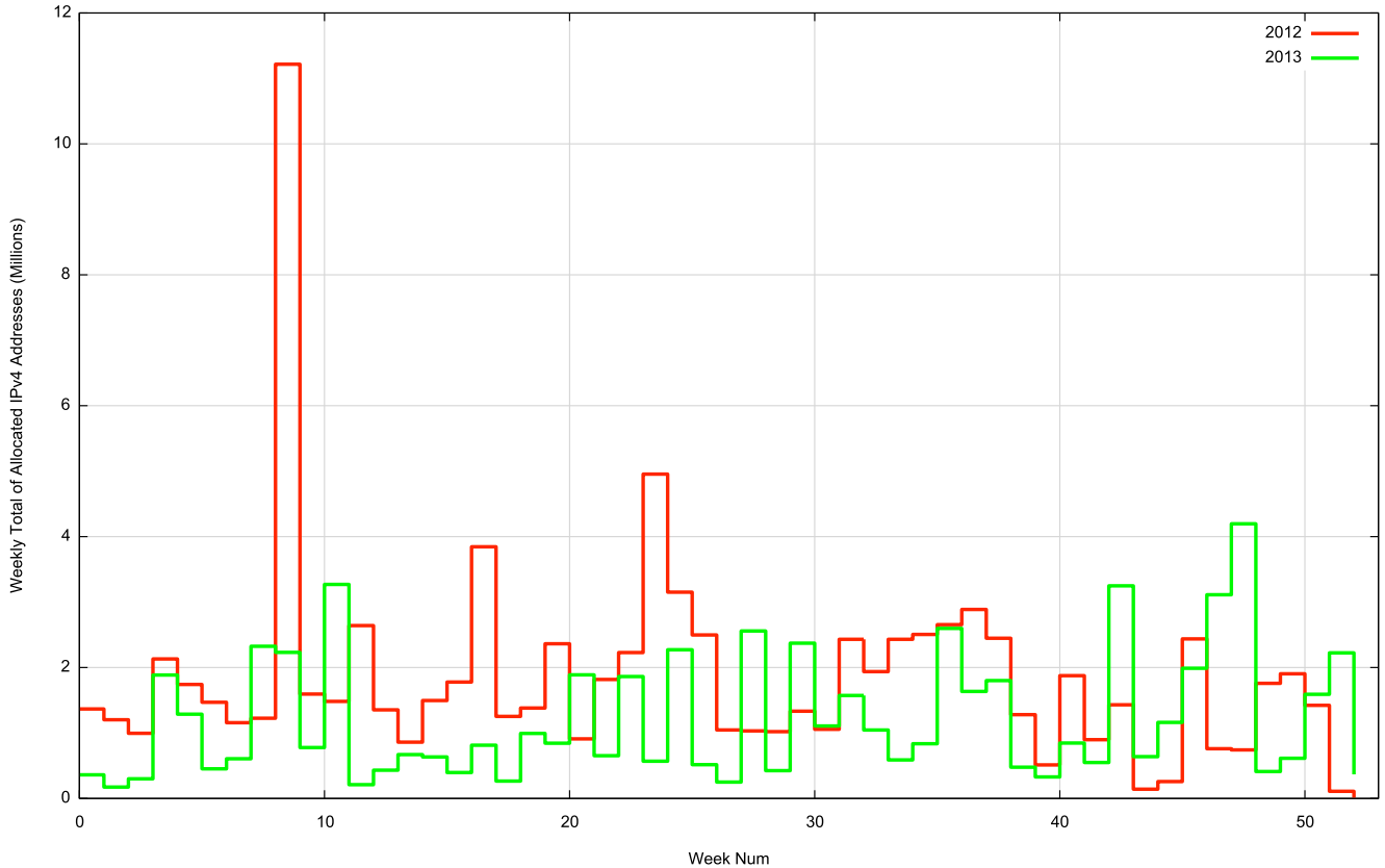
IPv4 Weekly Allocations
